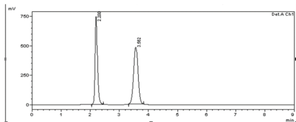
Figure 3. Chromatogram for linearity level of 10:100µg/ml
