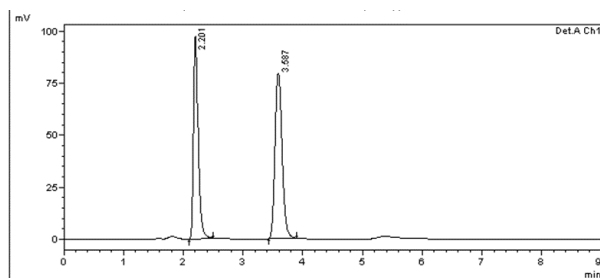
Figure 2. Chromatogram for linearity level 0.032:0.32µg/ml
