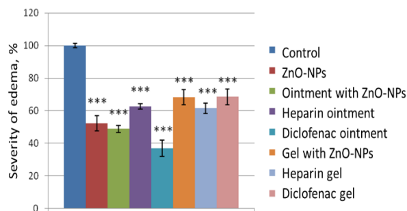
Figure 1. The effect of control and experimental substances on the severity of formalin edema of the paws of mice. Note: *, ** and *** – the differences with the control are significant at p < 0.05 , 0.01 and 0.001, respectively
